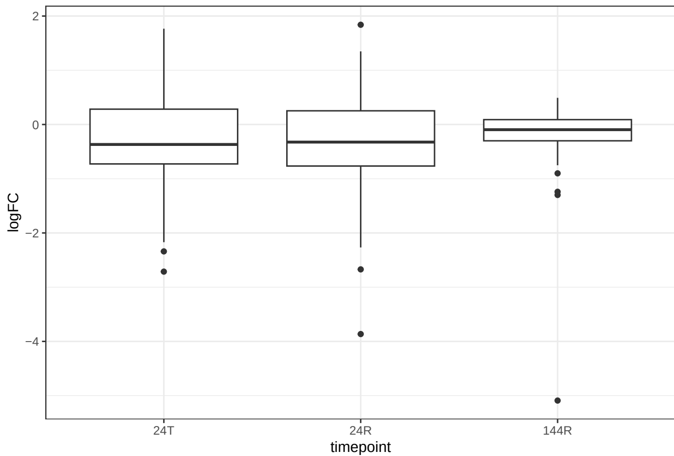
LFC at timepoints of nearest gene to MER61E TE elements in my data (GREAT)
